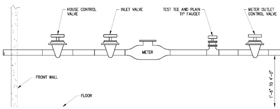
1"-2" DOMESTIC SERVICE WITH FIRE PROTECTION SPRINKLERS FOR SINGLE-JET OR ELECTRONIC METER FIGURE NO. 8
