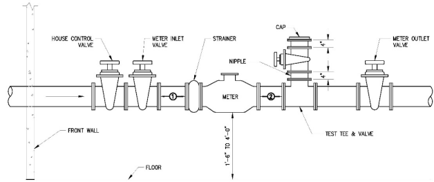
TYPICAL FOR TURBINE, SINGLE-JET, OR ELECTRONIC METERS FIGURE 9 (N.T.S.)
