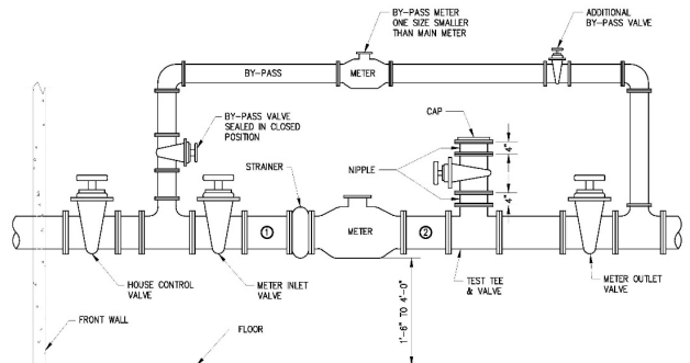
TYPICAL METER SETTING WITH BY-PASS (N.T.S.) TYPICAL FOR TURBINE, SINGLE-JET OR ELECTRONIC METERS FIGURE 10
