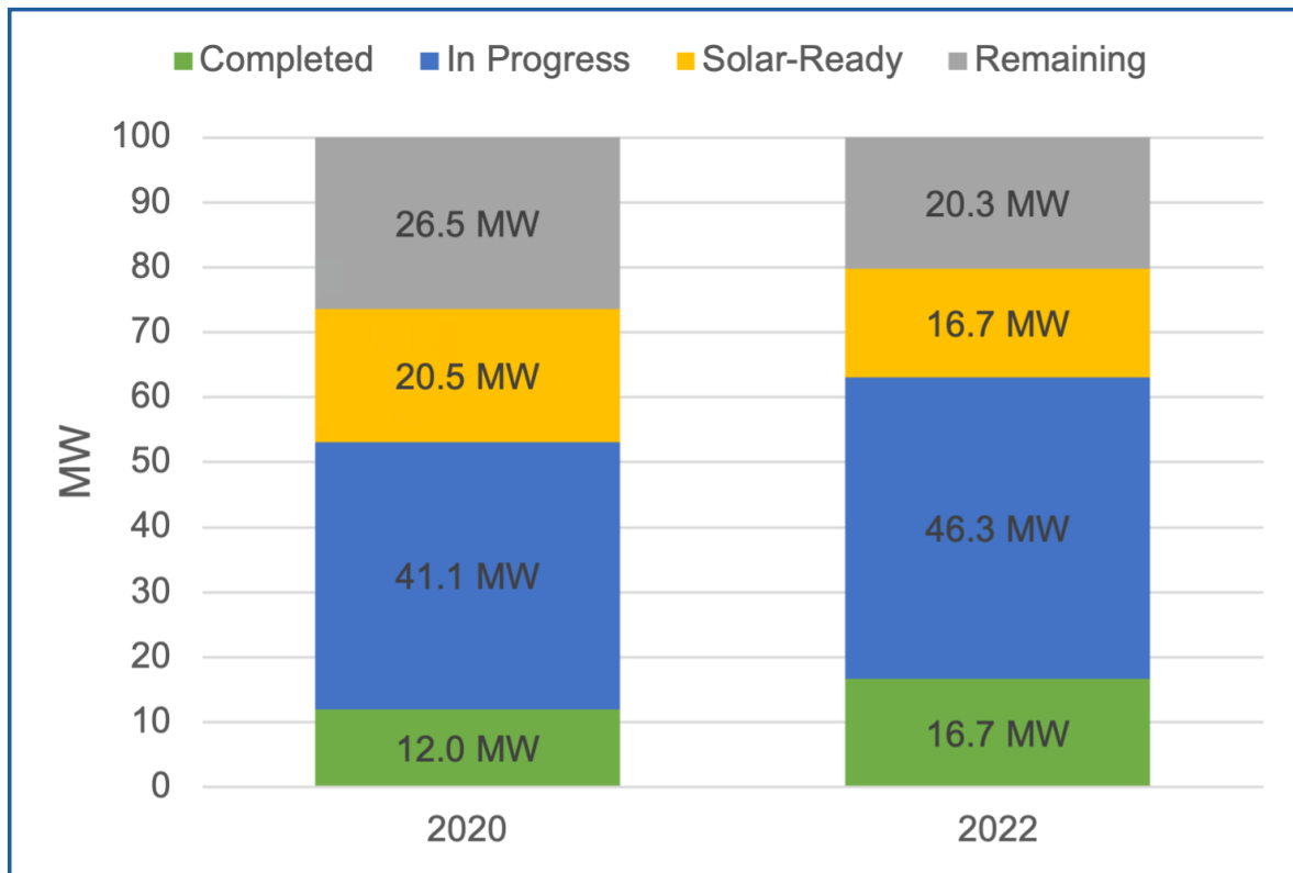
Figure 2. Progress Towards 100 MW – 2020 vs. 2022
