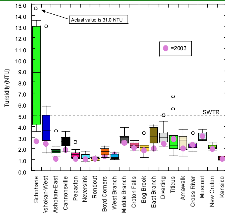
Figure 3.16 Annual median turbidity in NYC water supply reservoirs (2003 vs. 1993–2002).
