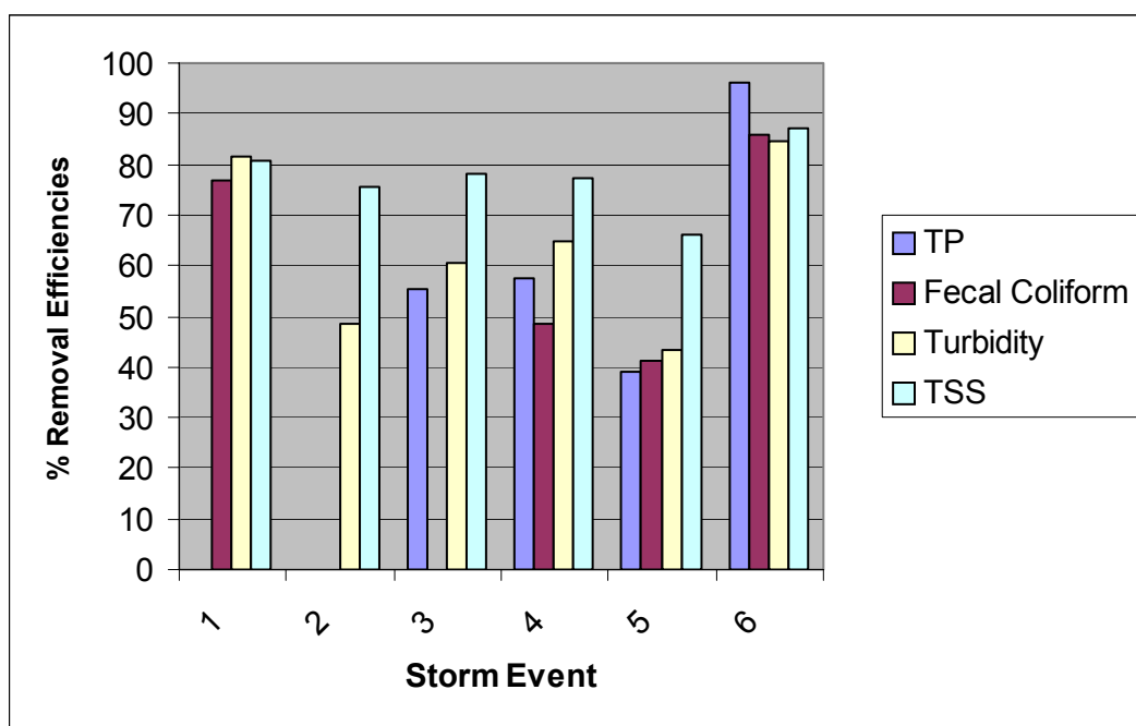
Figure 4.11 Pollutant removal efficiencies documented at Kensico Reservoir BMP 37.
