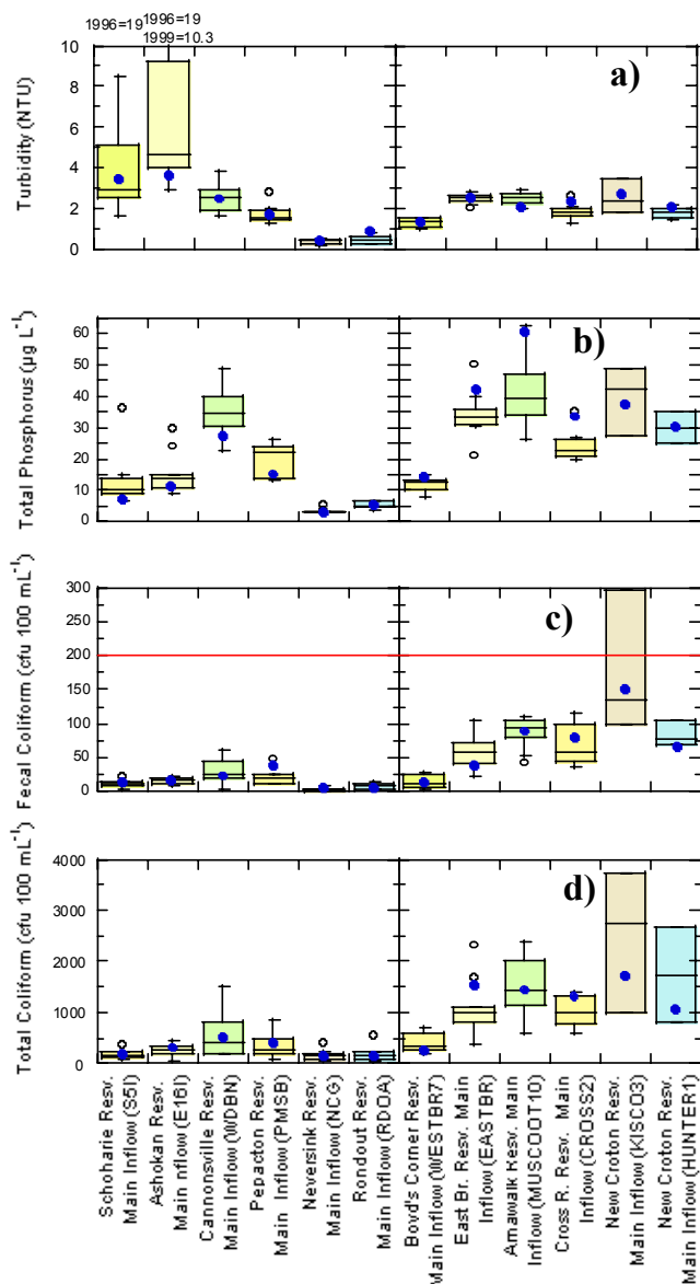
Figure 3.14 Box plot of annual medians (1993–2002) for a) turbidity, b) total phosphorus, c) fecal coliforms, d) total coliforms for selected stream (reservoir inflow) sites with the value for 2003 displayed as a dot.
