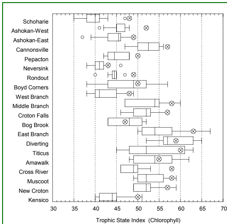
Figure 3.23 Box plots of annual Trophic State Index (1993–2002) and 2003 value (as x) for New York City reservoirs, based on chlorophyll a concentration.
