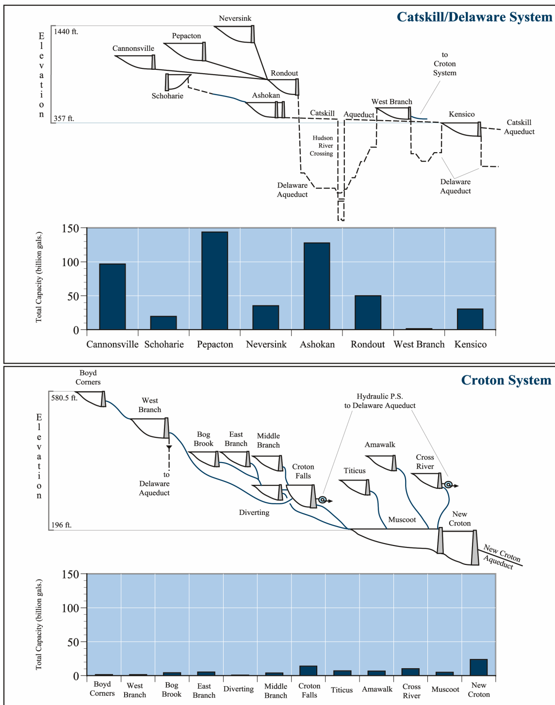
Figure 2.2 NYC water supply reservoirs and their available storage capacities.
