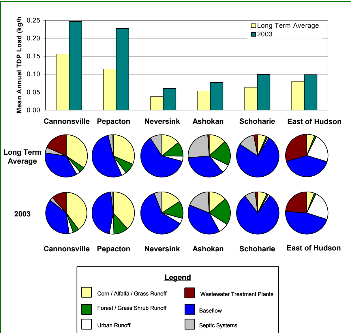
Figure 5.3 Relative simulated contributions of various non-point source land uses and point sources to TDP loads to the reservoirs for 2003 in relation to long-term simulated annual statistics.
