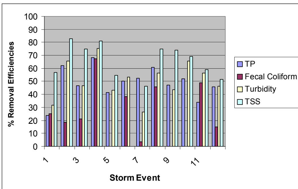
Figure 4.10 Pollutant removal efficiencies documented at Kensico Reservoir BMP 12.
