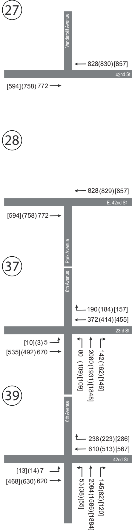
FIGURE 15-21a | Future Conditions With the Proposed Action AM, Midday, and PM Peak Hour Volumes (Manhattan-East)
