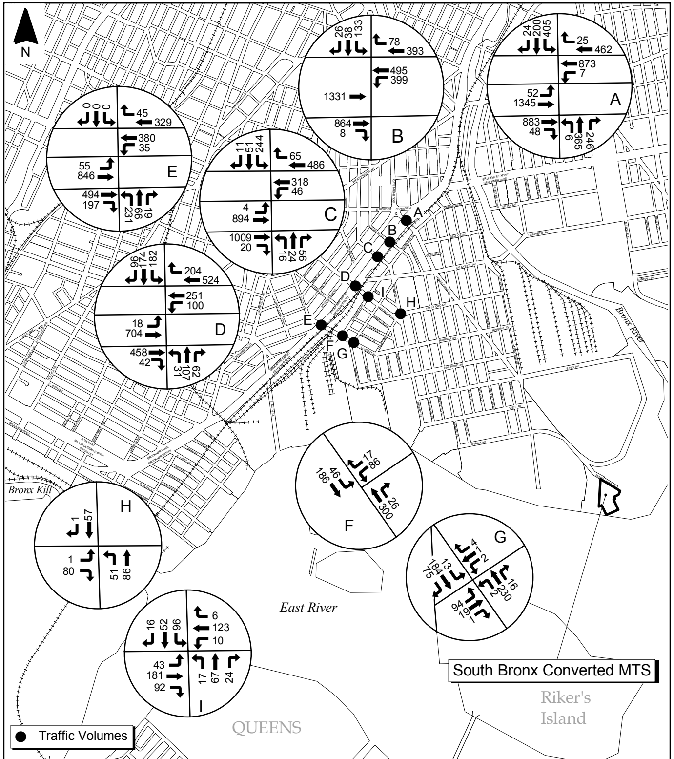
Figure 19.14-20 2006 Future Build Traffic Volumes PM Peak South Bronx Converted MTS CITY OF NEW YORK DEPARTMENT OF SANITATION
