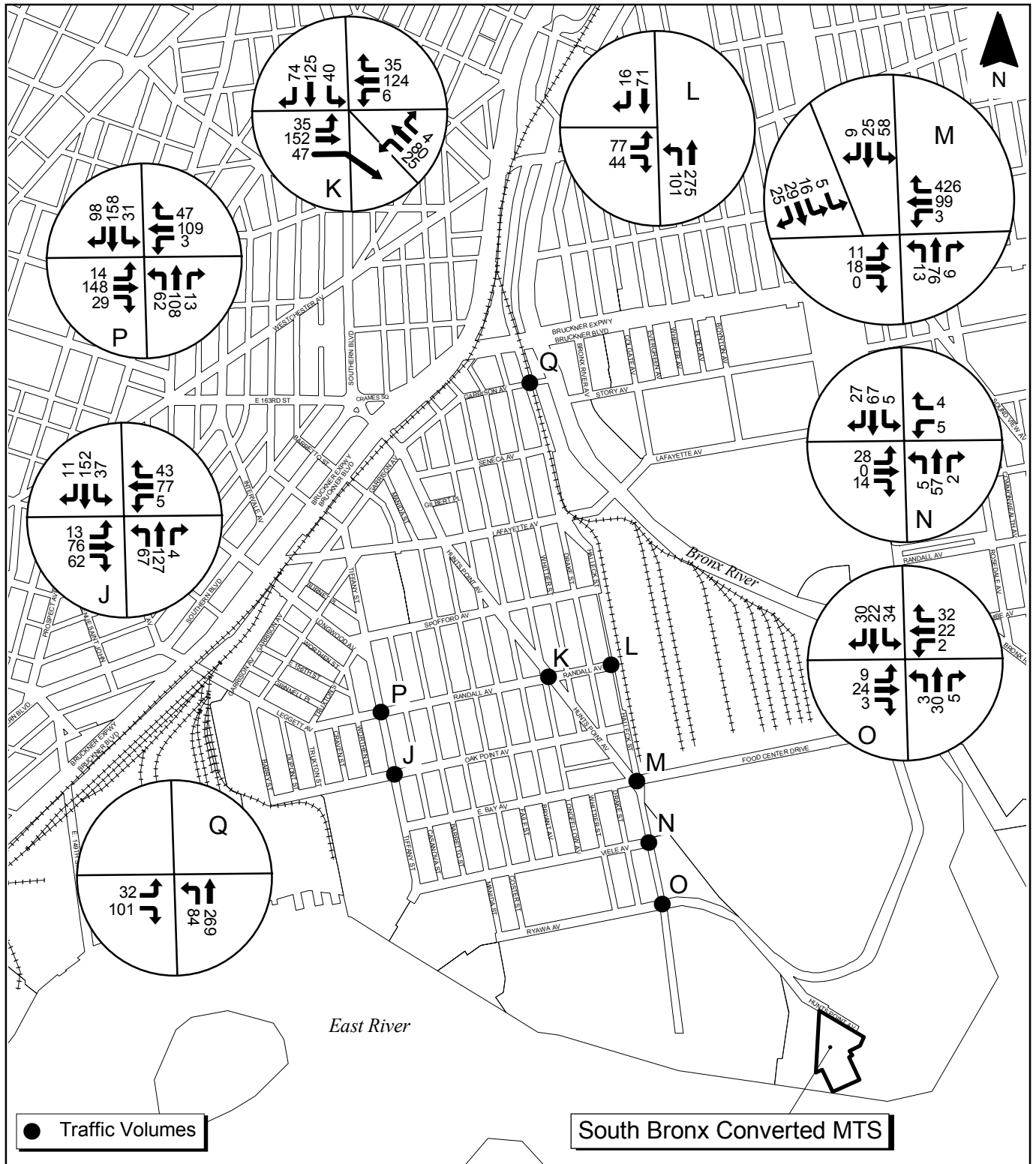
Figure 19.14-5 Existing Traffic Volumes Facility Peak South Bronx Converted MTS CITY OF NEW YORK DEPARTMENT OF SANITATION
