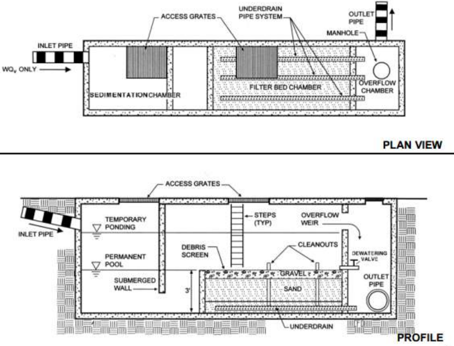
Figure 6-7. Plan and Profile Views of the Sand Filter Standard Design Developed by NYS DEC
