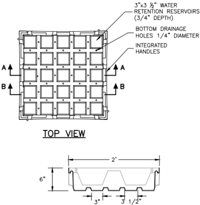
Figure 6-10. Dimensions of the 6" Deep Modular Green Roof Tray
