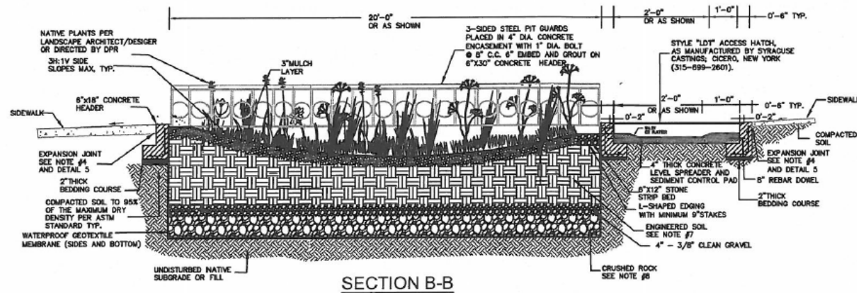
Figure 6-4: DEP Standard Design for a Bioretention Practice with Underdrain and Permeable Pavement
