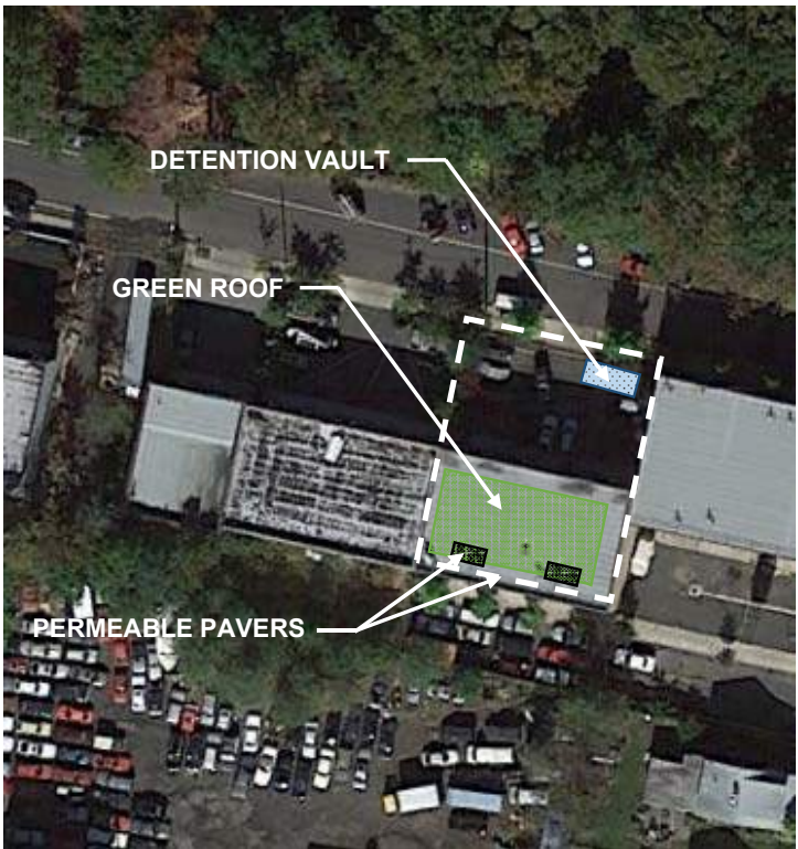
SITE SCHEMATIC with STORMWATER CONTROL MEASURE (SCM)
