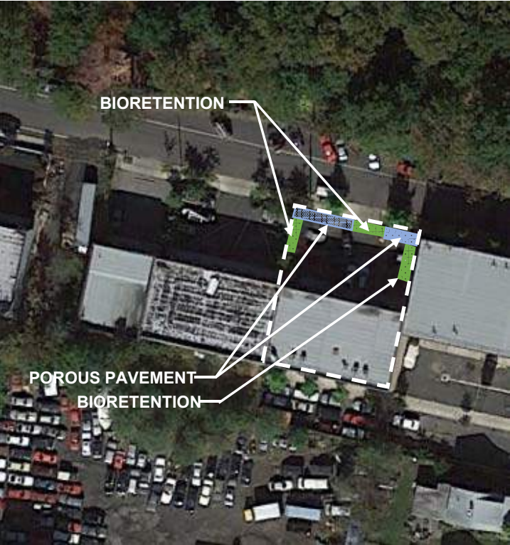
SCM SCHEMATIC
