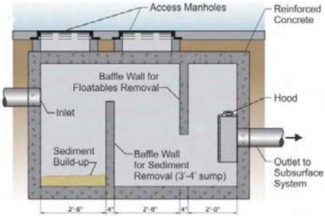
Pretreatment Structure
