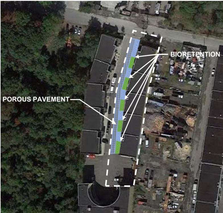
SCM SCHEMATIC
