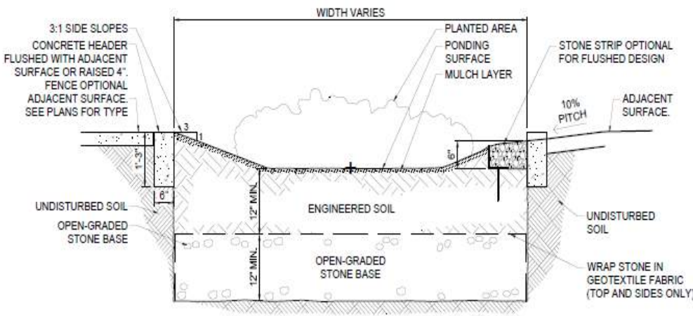
Figure 6-2: DEP Standard Design for a Bioretention Practice
