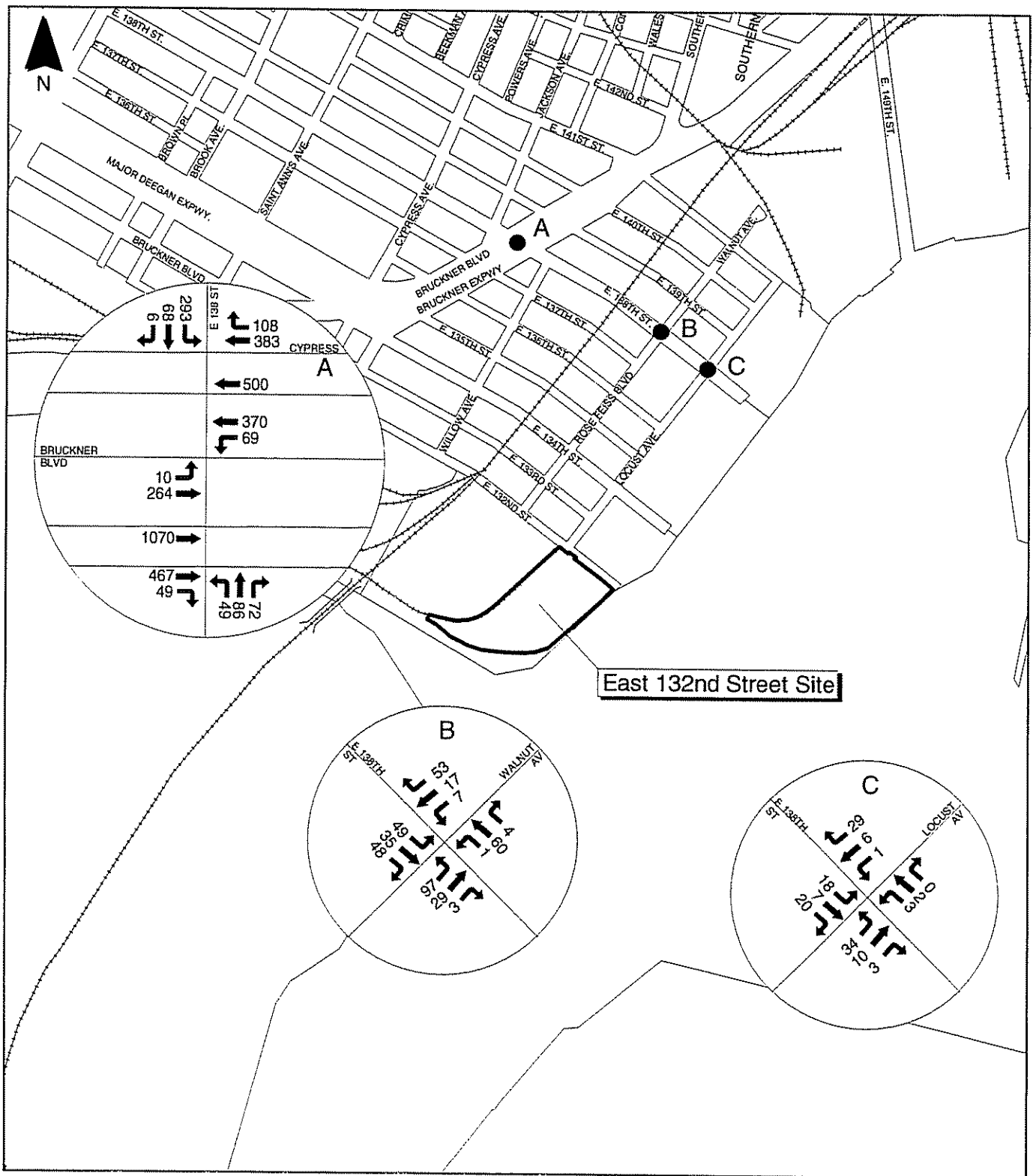
Figure 12.14-3 Existing Traffic Volumes Facility Peak East 132nd Street Site
