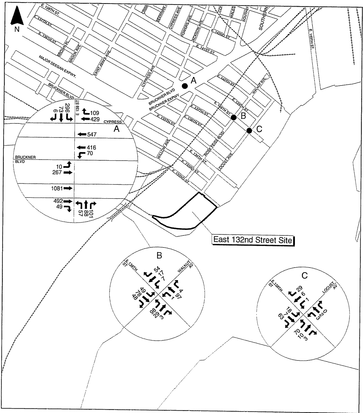
Figure 12.14-12 2006 Build Traffic Volumes Facility Peak East 132nd Street Site
