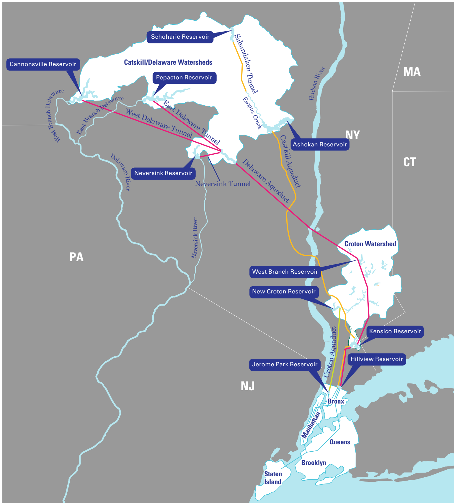
WATER DELIVERY SYSTEM (SOURCE: NYC DEP, 2011)
