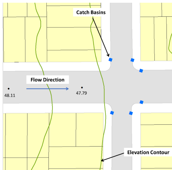
Figure 6.1. Example roadway flow direction analysis.
