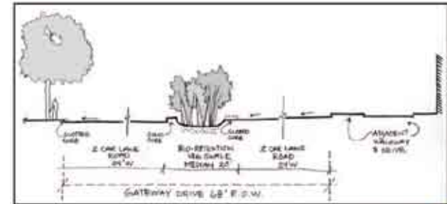
Gateway Drive Section = N.T.S.
