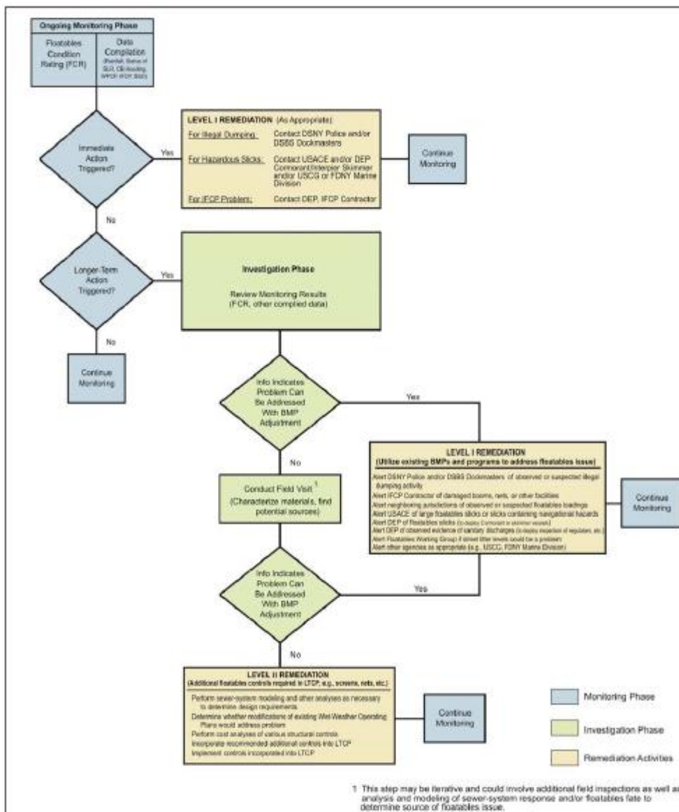
Figure 7. Pilot floatables monitoring program monitoring/remediation flow chart.
