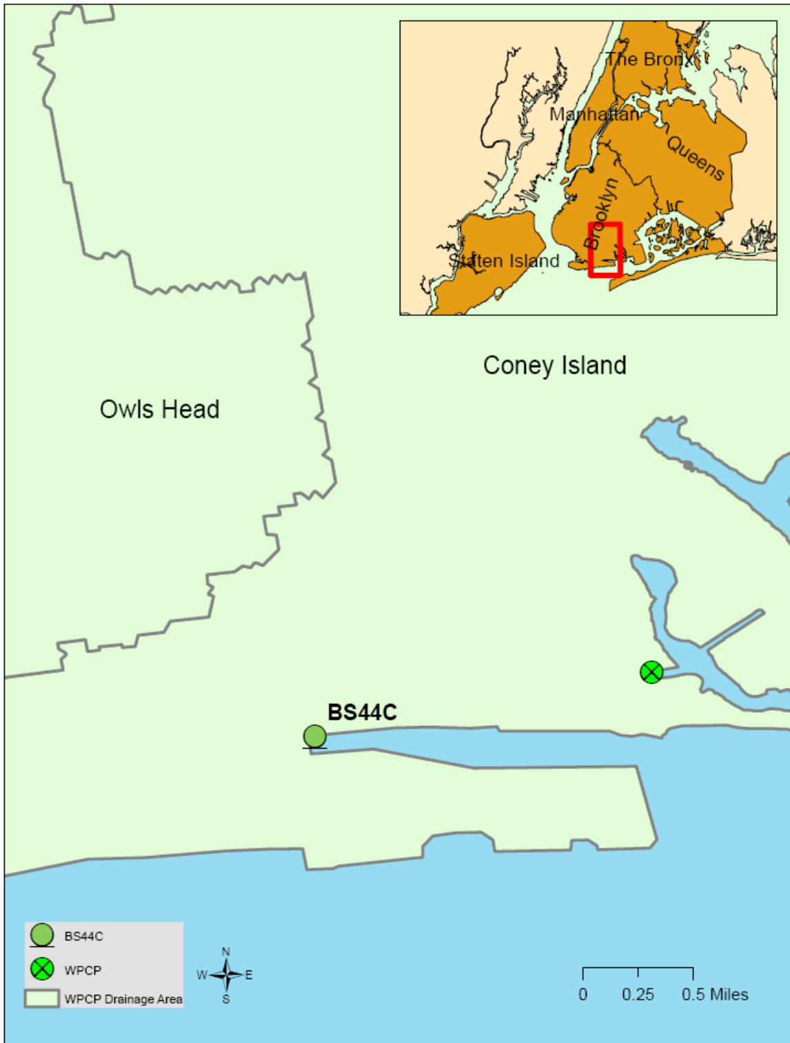
Figure 20. Drainage Area map of the Holocaust Memorial (BS44C) area. The site drains to Coney Island Treatment Plant.
