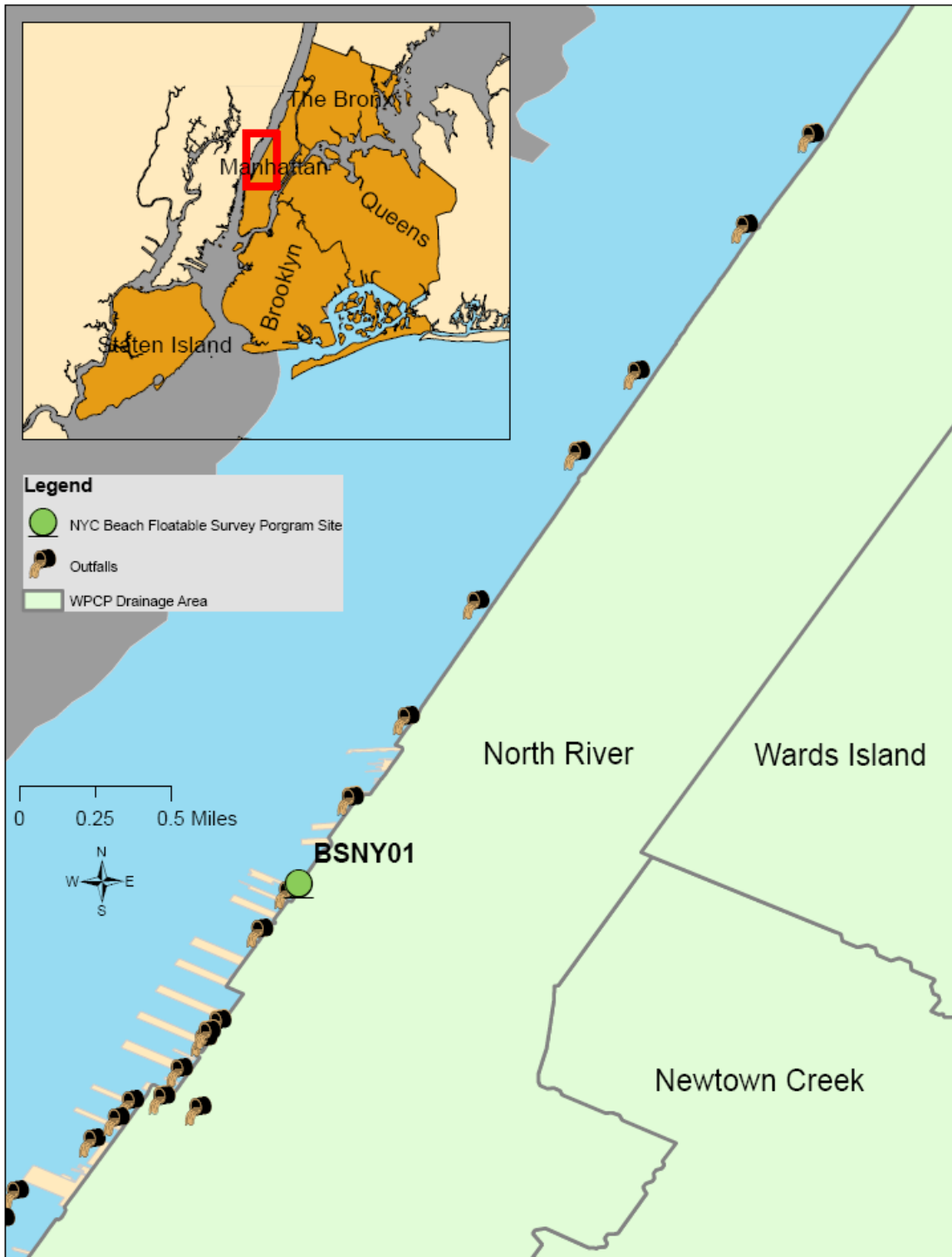
Figure 26. Drainage area map of the Pier 99 (BSNY01) area. The site lies in the North River WWTP drainage basin.
