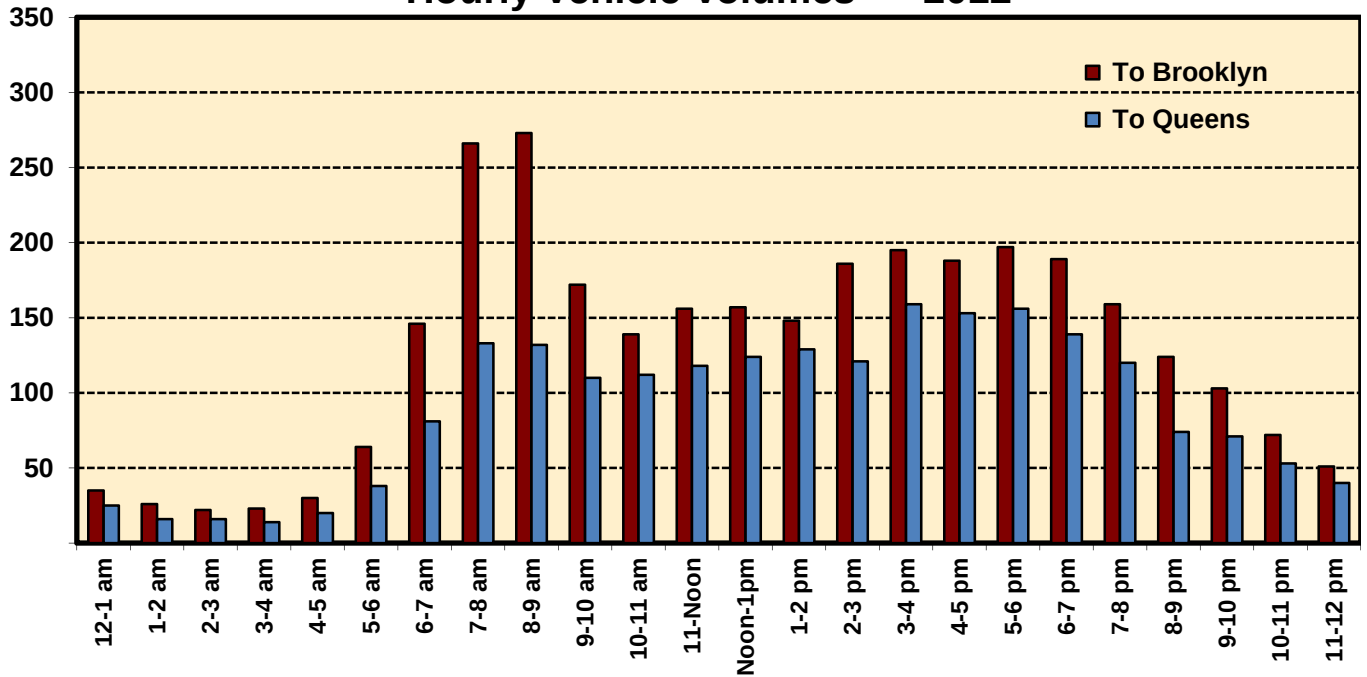
DeKalb Avenue Hourly Vehicle Volumes ~ 2012
