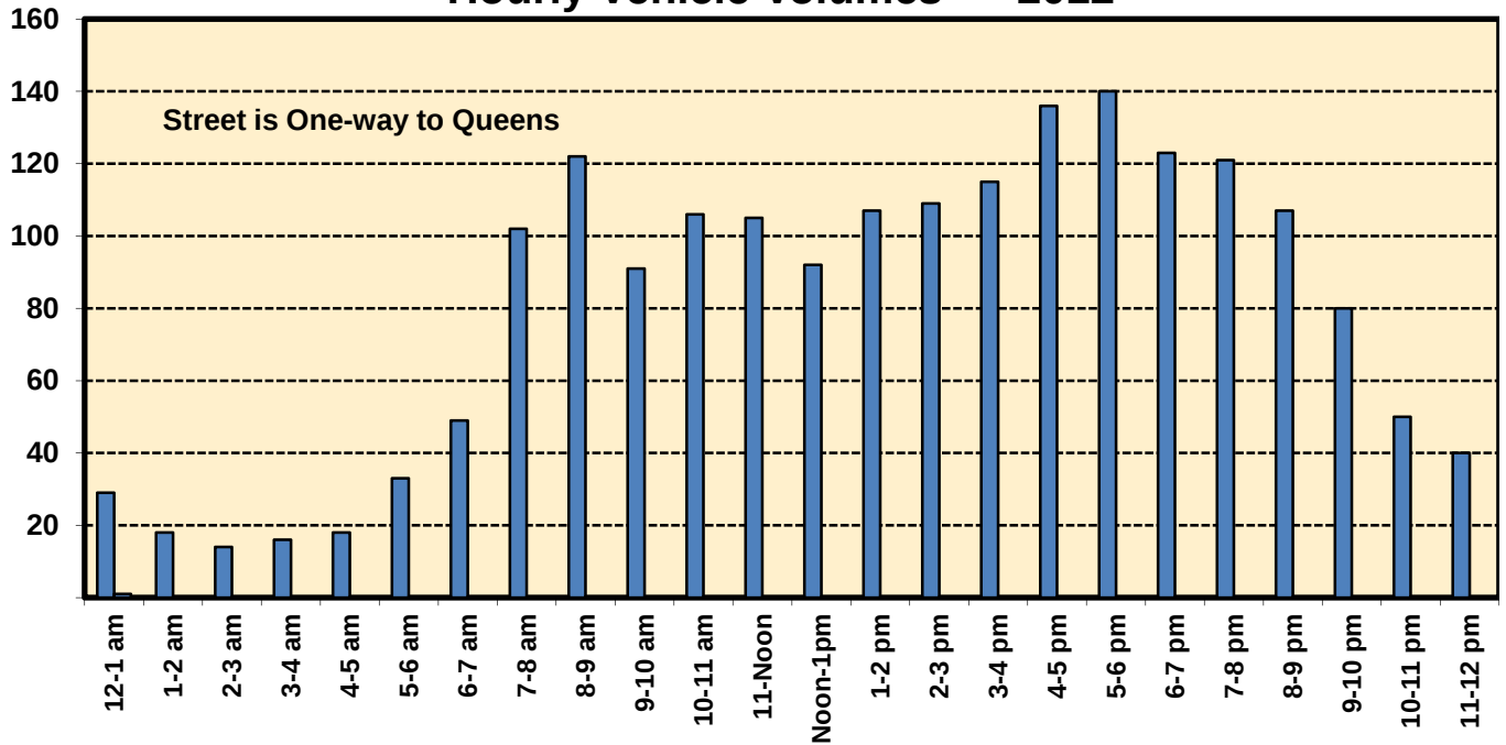
Linden Street Hourly Vehicle Volumes ~ 2012
