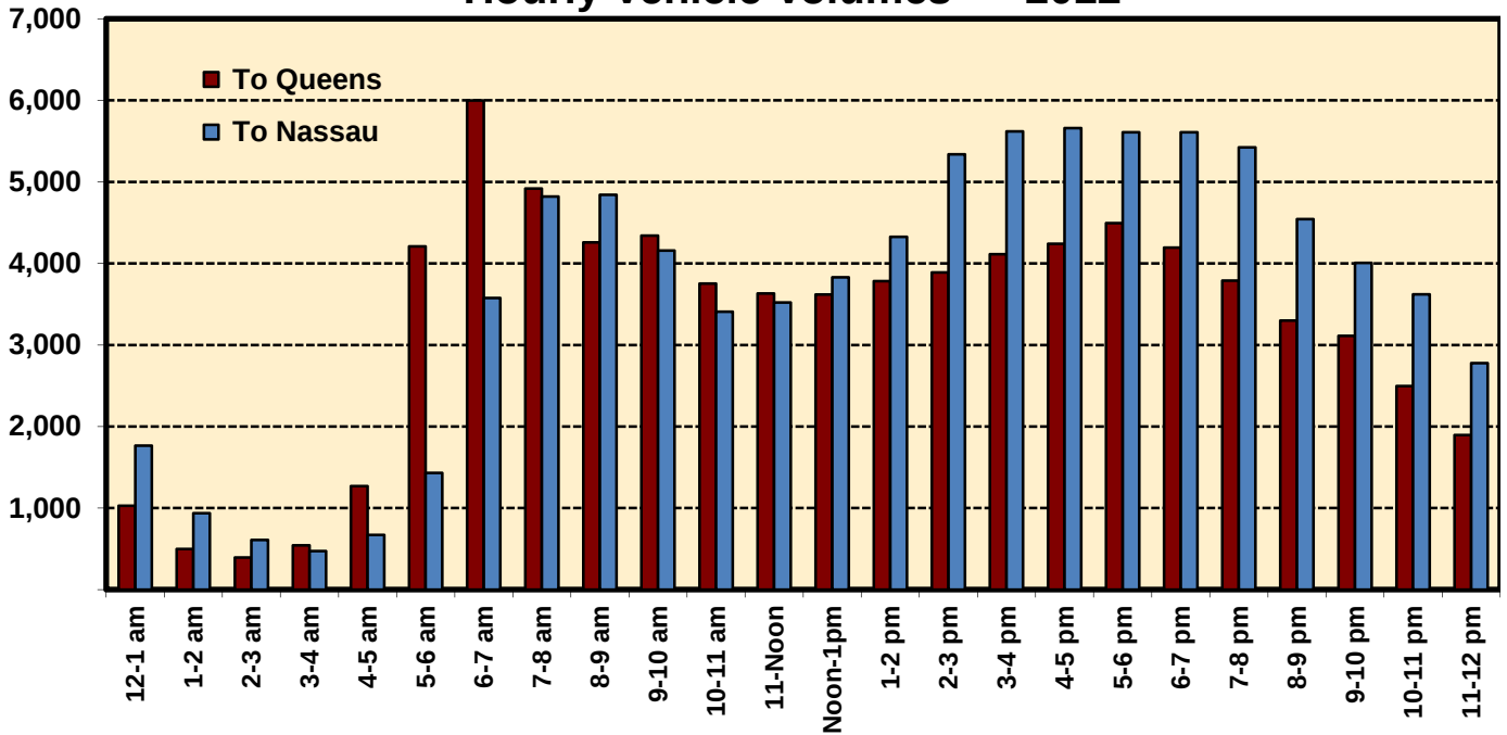
Laurelton Parkway Hourly Vehicle Volumes ~ 2012
