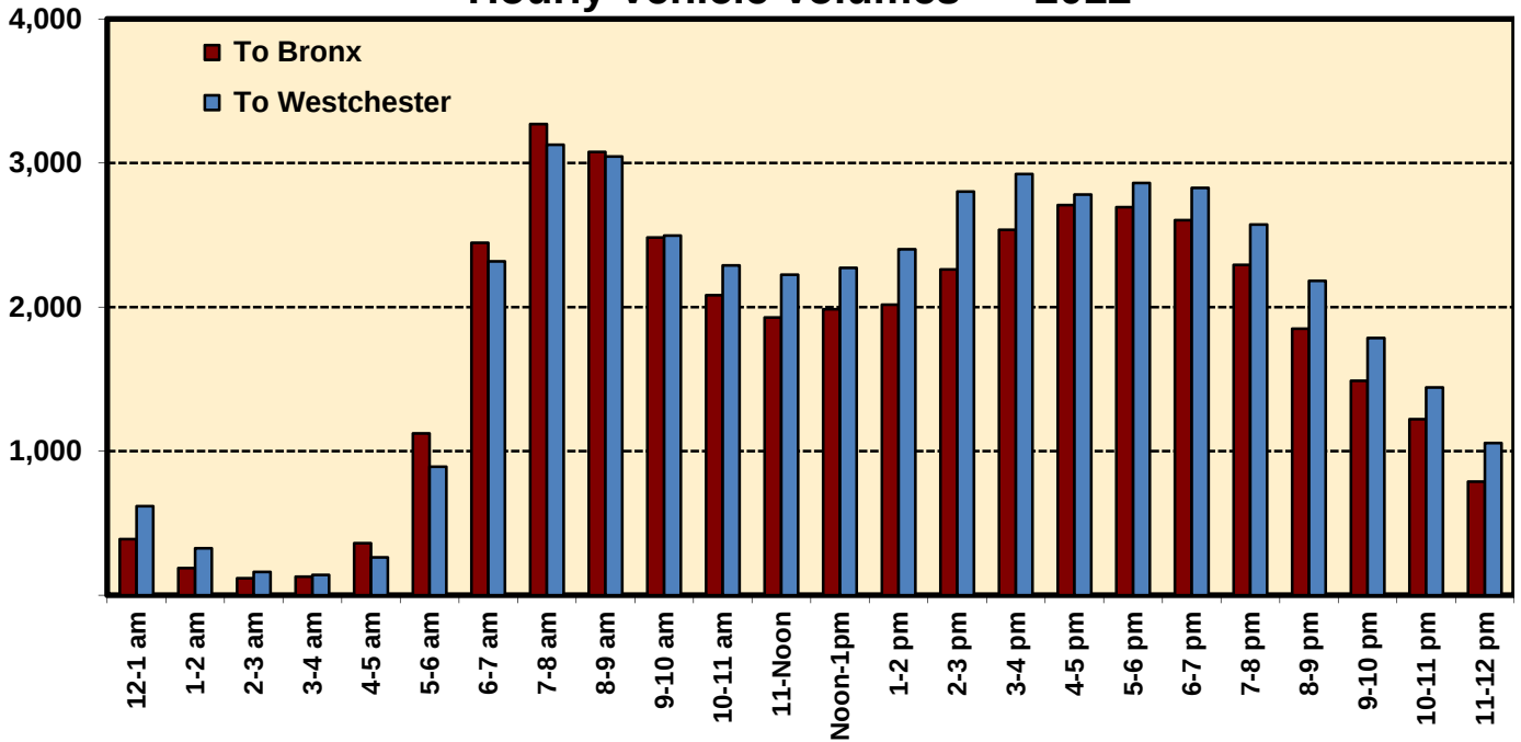
Hutchinson River Parkway Hourly Vehicle Volumes ~ 2012
