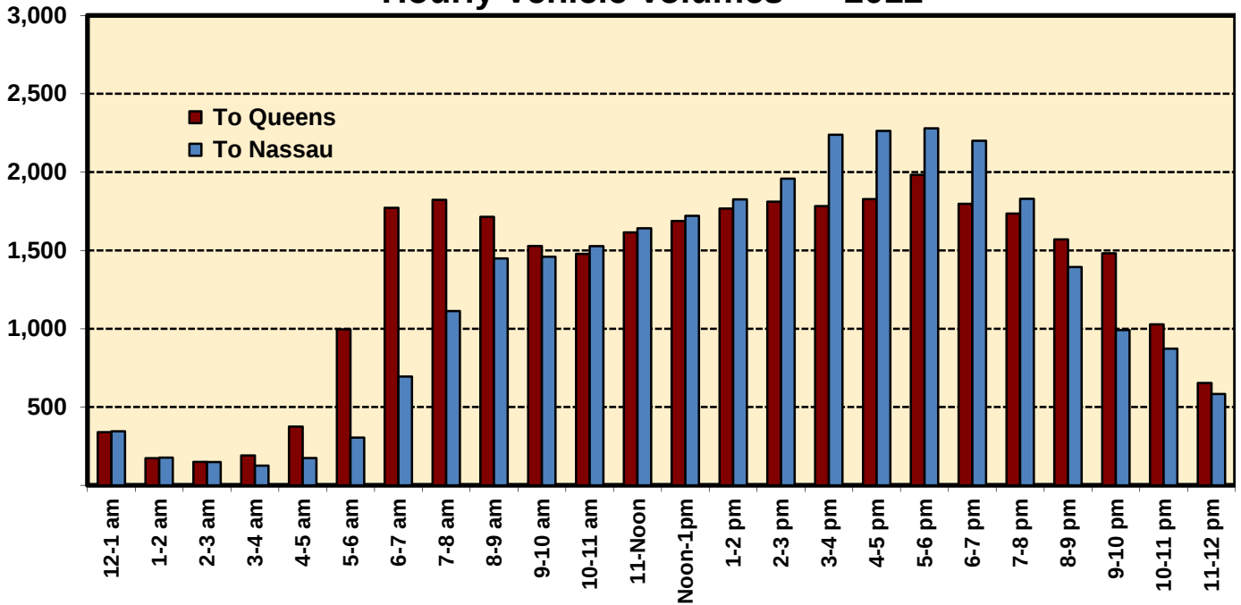
Sunrise Highway Hourly Vehicle Volumes ~ 2012
