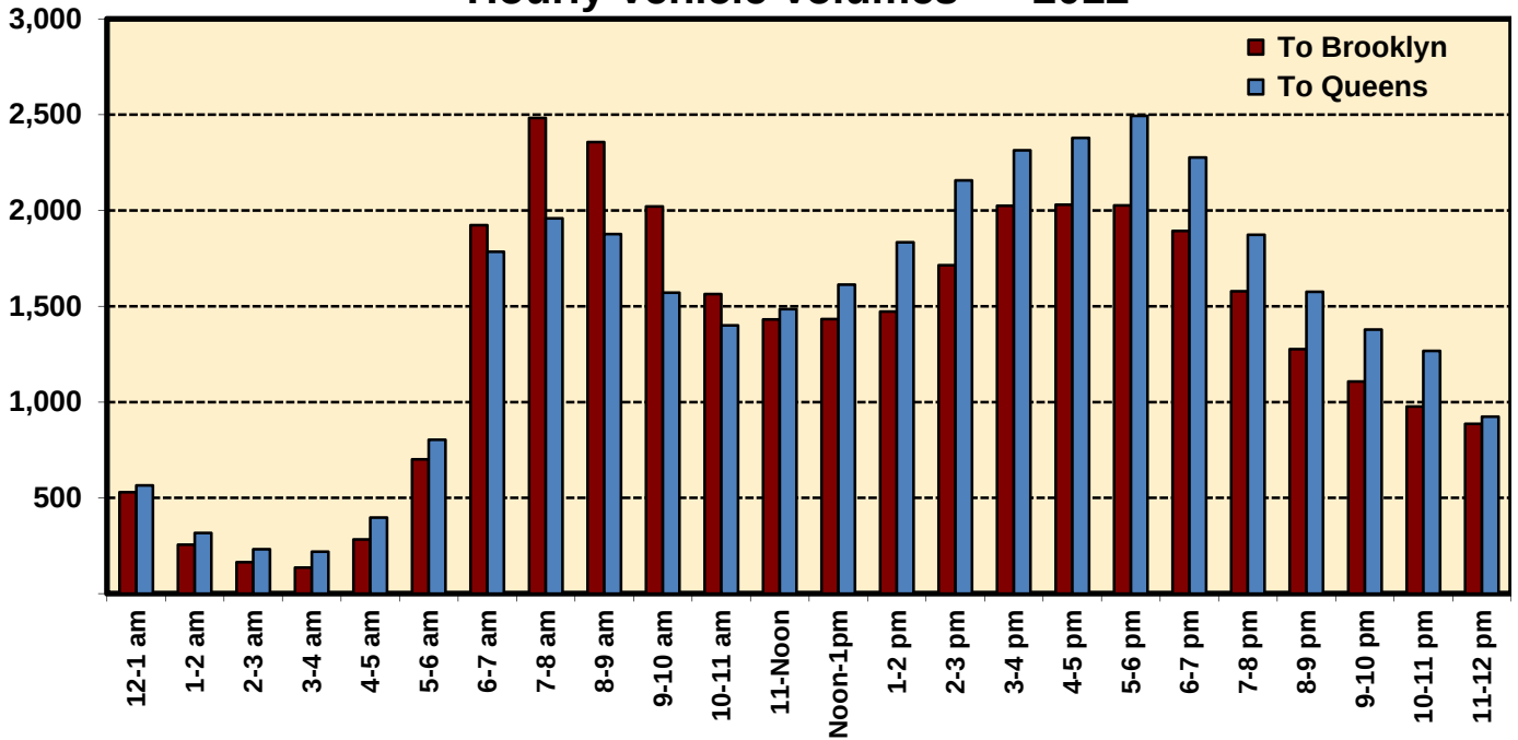
Jackie Robinson Parkway Hourly Vehicle Volumes ~ 2012
