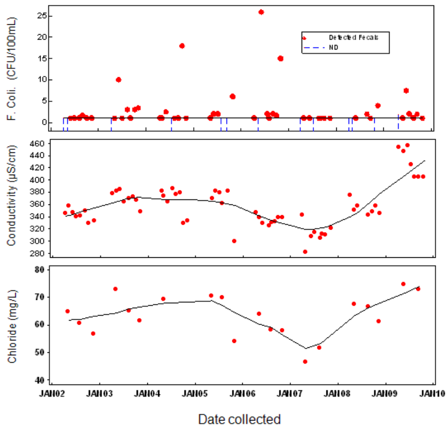
Figure 3.22 New Croton Reservoir temporal plots of selected water quality analytes. Red dots are monthly medians. The black line on the fecal coliform plot is the Akritas-Theil-Sen line, while the dashed blue lines indicate non-detects. On the conductivity and chloride plots the black line is a LOWESS curve with a 30% smooth factor. Fecal coliform and conductivity medians were calculated using samples collected at all sites and depths and represent whole reservoir conditions. Chloride medians were calculated from all depths collected at Site 1.
