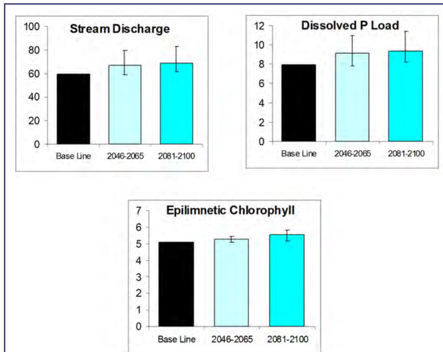
Figure 6.5 Total annual streamflow, and dissolved phosphorus loading compared with the mean annual reservoir chlorophyll a concentration. For the future time periods, the solid bar shows the median and vertical lines show the range of nine simulations.
