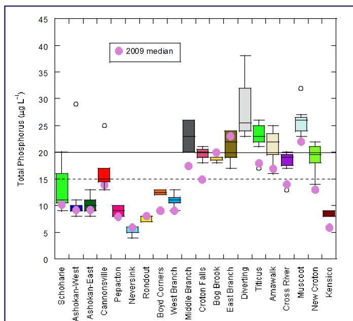
Figure 3.7 Annual median total phosphorus in NYC water supply reservoirs (2009 vs. 2002-2008). The horizontal dashed line at 15 \mu\text{g L}^{-1} refers to the NYC TMDL guidance value for source waters. The horizontal solid line at 20 \mu\text{g L}^{-1} refers to the NYSDEC ambient water quality guidance value appropriate for reservoirs other than source waters (the remaining reservoirs).
