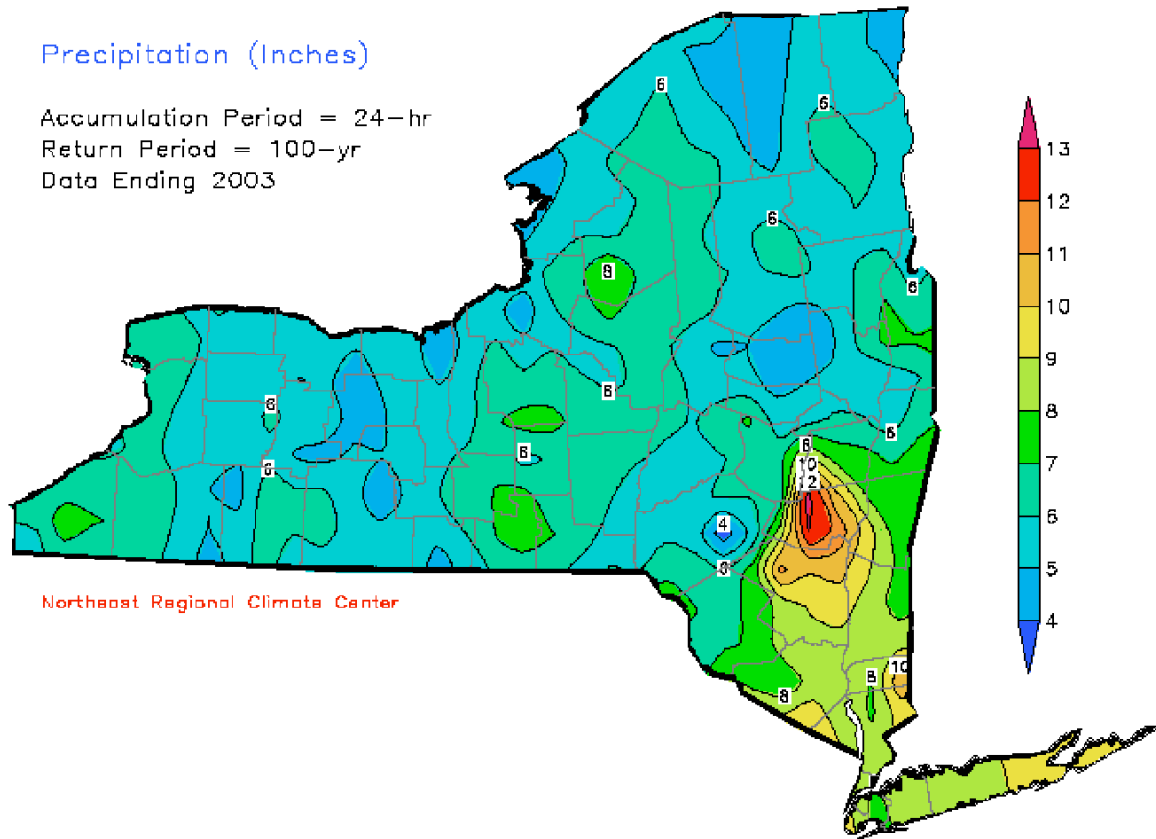
Figure 2.8 The 100-year, 24-hour storm for New York State as determined by the Northeast Regional Climate Center ( http://www.nrcc.cornell.edu/pptext/isomaps.html ).
