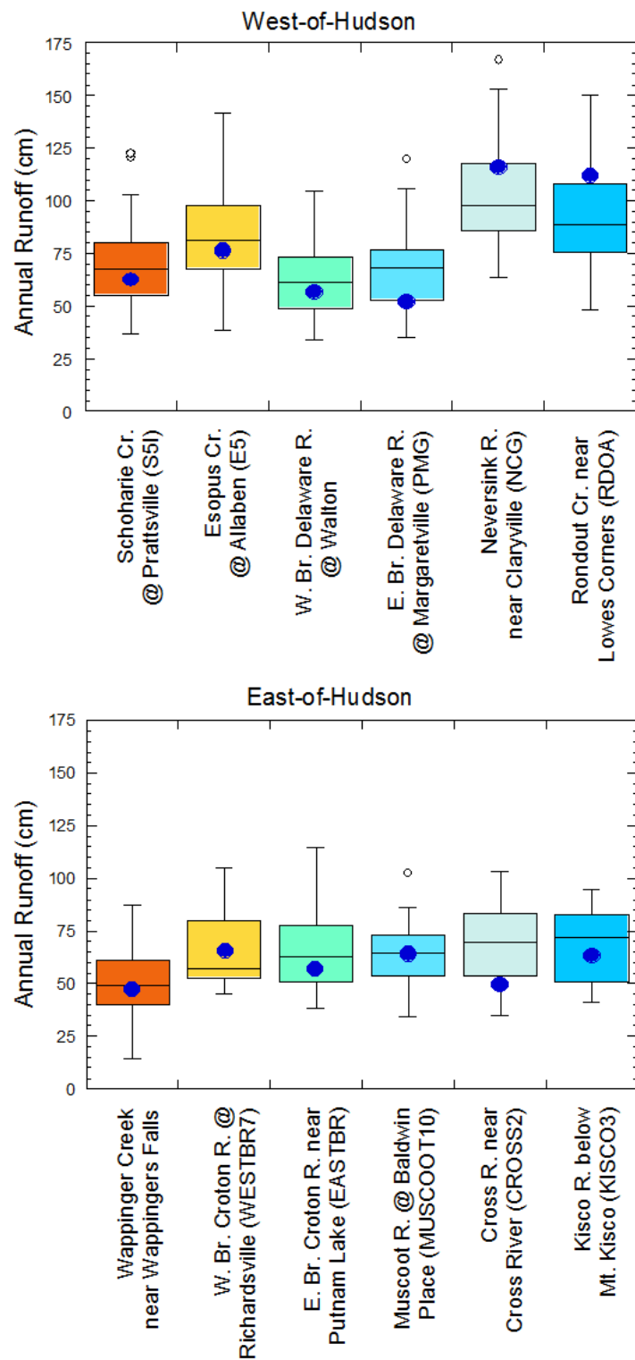
Figure 2.3 Historical annual runoff (cm) as boxplots for the WOH and EOH watersheds, with the values for 2009 displayed as a dot.
