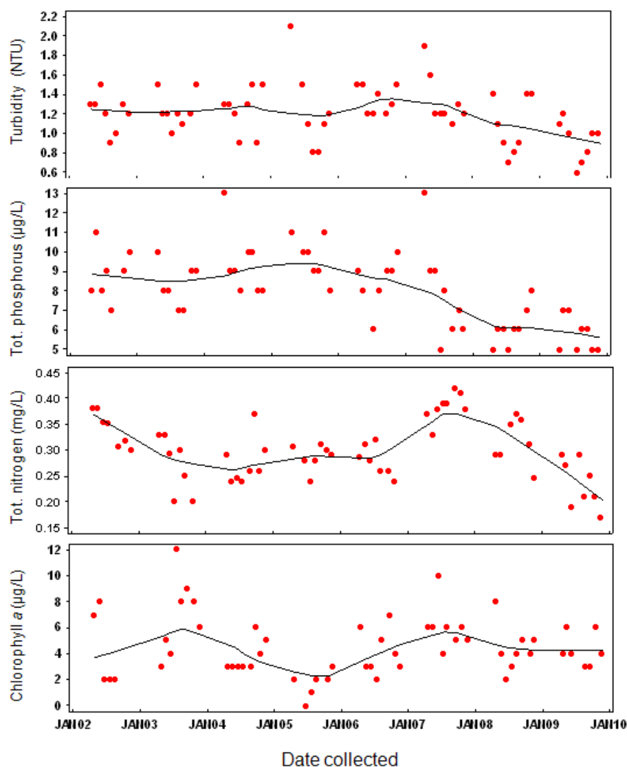
Figure 3.19 Kensico Reservoir temporal plots of selected water quality analytes. Red dots are monthly medians. The black line is a LOWESS curve with a 30% smooth factor. Chlorophyll medians were calculated from samples collected at all sites at a depth of 3 meters and represent surface water conditions. Turbidity, total phosphorus, and total nitrogen medians were calculated from all sites and depths and represent whole reservoir conditions.
