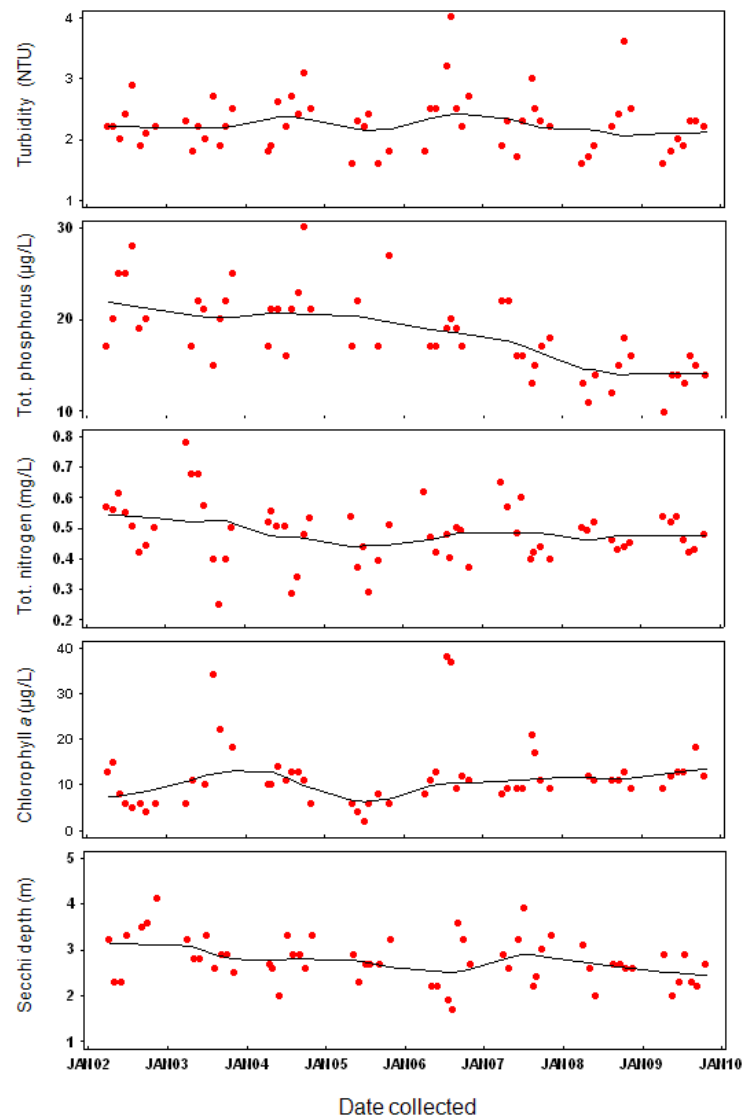
Figure 3.21 New Croton Reservoir temporal plots of selected water quality analytes. Red dots are monthly medians. The black line is a LOWESS curve with a 30% smooth factor. Chlorophyll and Secchi depth medians are representative of surface water conditions. Turbidity, total phosphorus, and total nitrogen medians were calculated from all sites and depths and represent whole reservoir conditions.
