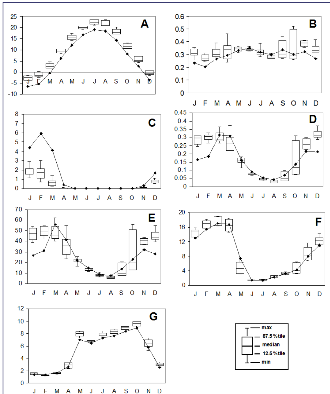
Figure 6.3 Average conditions for present day (solid line) and a range of future conditions (bar) for Cannonsville Reservoir and watershed. A) Mean daily air temperature ( ^{\circ}\text{C} ), B) Mean daily precipitation (cm), C) Mean snow pack water equivalent (cm), D) Mean daily stream discharge (cm), E) Mean reservoir dissolved phosphorus export ( \text{kg km}^{-2} \text{mo}^{-1} ), F) Mean reservoir dissolved phosphorus concentration ( \text{mg m}^{-3} ), G) Mean reservoir chlorophyll a concentrations ( \text{mg m}^{-3} ).
