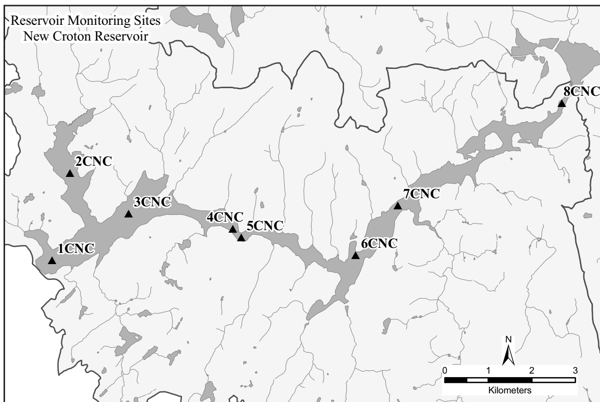
Appendix Figure F.2 Sites included in the trends analysis for New Croton Reservoir.
