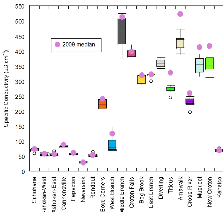
Figure 3.12 Annual median specific conductivity in NYC water supply reservoirs (2009 vs. 2002-2008). Specific conductivity is conductivity at 25°C.
