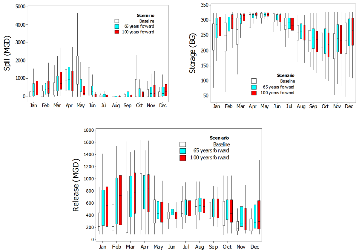
Figure 6.6 Monthly WOH storage, controlled release, and uncontrolled spill to downstream rivers for baseline and 65 and 100 years forward. Middle lines represent the median, boxes the 25 th and 75 th interquartile range.
