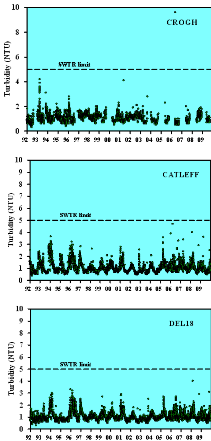
Figure 3.3 Turbidity at keypoints compared to Surface Water Treatment Rule limit, 1992–2009.
