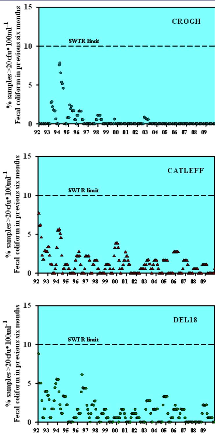
Figure 3.2 Fecal coliform (percent of daily samples > 20 CFU 100ml -1 in the previous six months) at keypoints compared to Surface Water Treatment Rule limit, 1992–2009.
