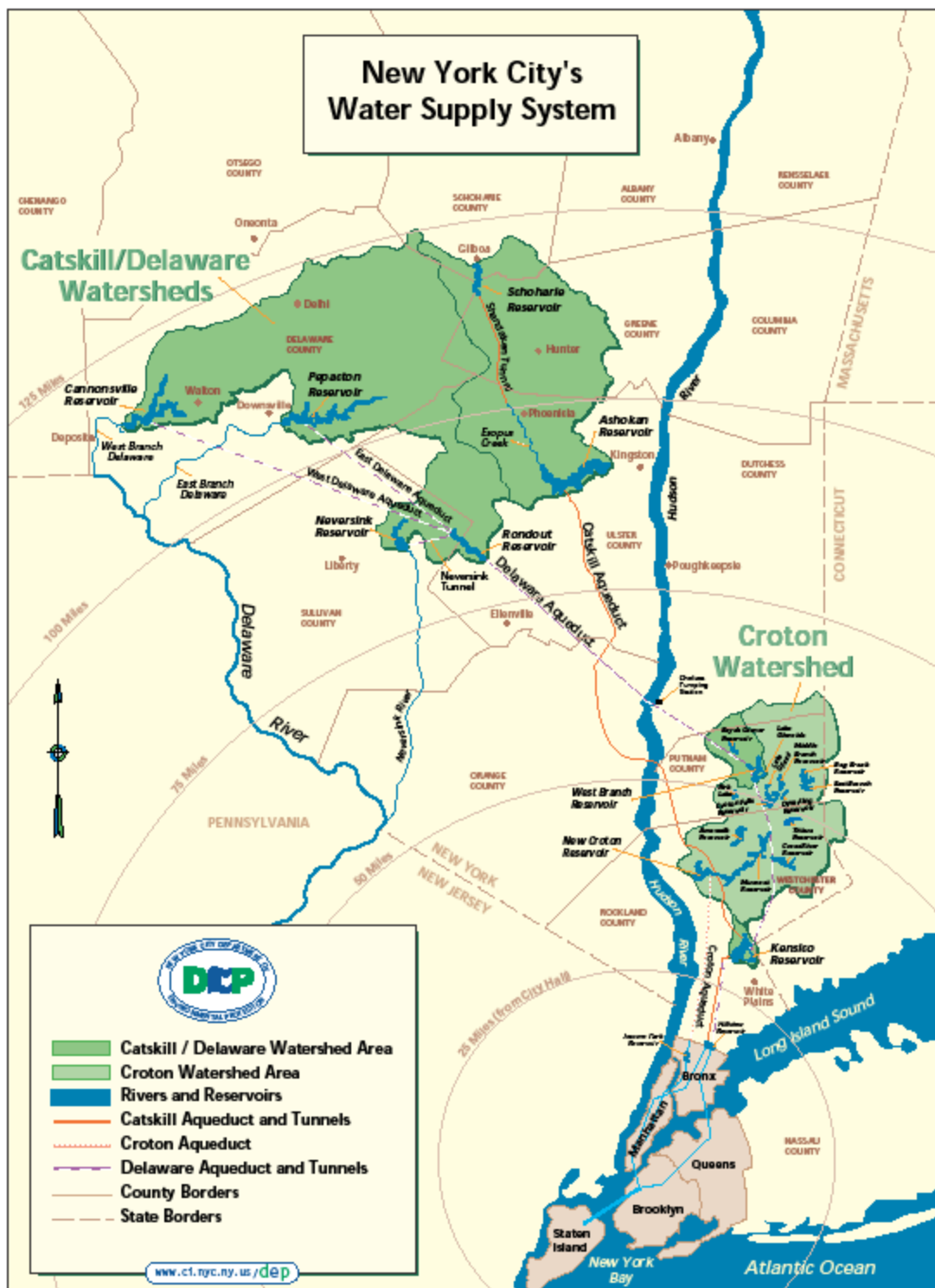
Figure 1.2 The New York City Water Supply System watersheds.
