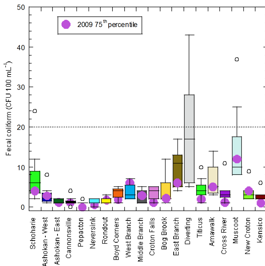
Figure 3.11 Annual 75 th percentile of fecal coliform in NYC water supply reservoirs (2009 vs. 2002-2008). The dashed line represents the SDWA standard for source waters as a reference.
