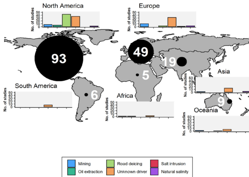
Figure 3: Global studies on salinization from 2017 to 2021. Circle size and white numbers correspond to the total number of studies conducted on each continent. 22
