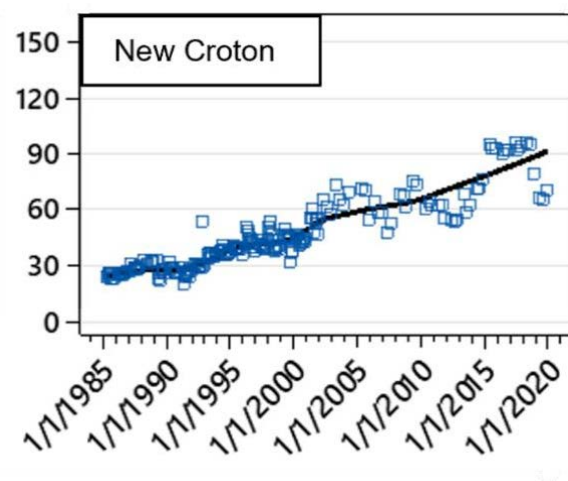
Figure 1: Temporal (1985-2019) chloride trend for New Croton Reservoir. Lines are LOWESS curves fitted through approximately monthly and quarterly data using a 30% smoothing factor.
