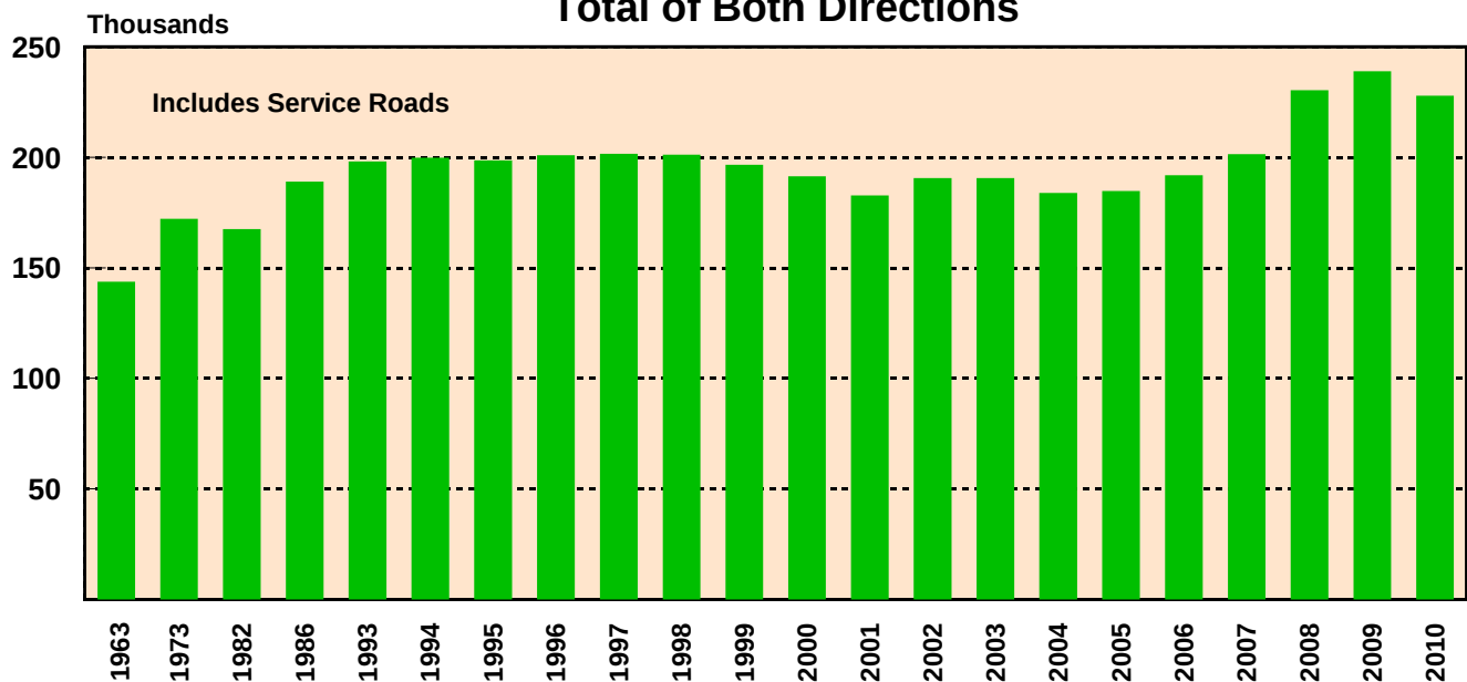
Long Island Expressway Average Daily Traffic Volumes Total of Both Directions
